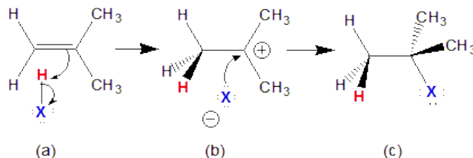
Figure 13.28: The Addition of a Hydrogen Halide Across a Double Bond
