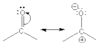
Figure 13.19: Resonance Forms of a Carbonyl Group
