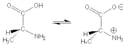
Figure 13.27: Alanine, an Amino Acid
