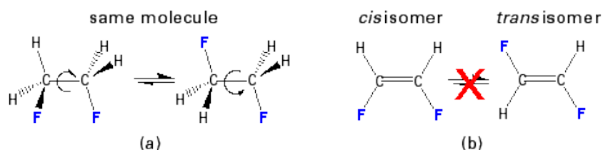
Figure 13.12: Rotation can occur about single bonds, but not about double bonds.
