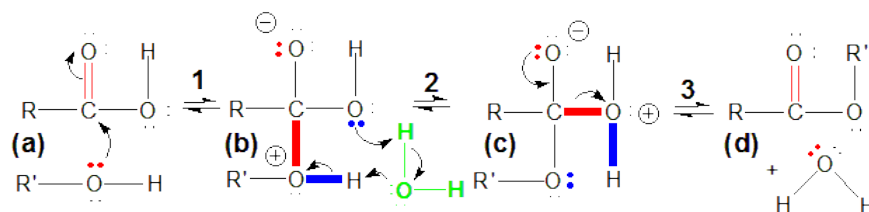
Figure 13.30: Esterification Mechanism
