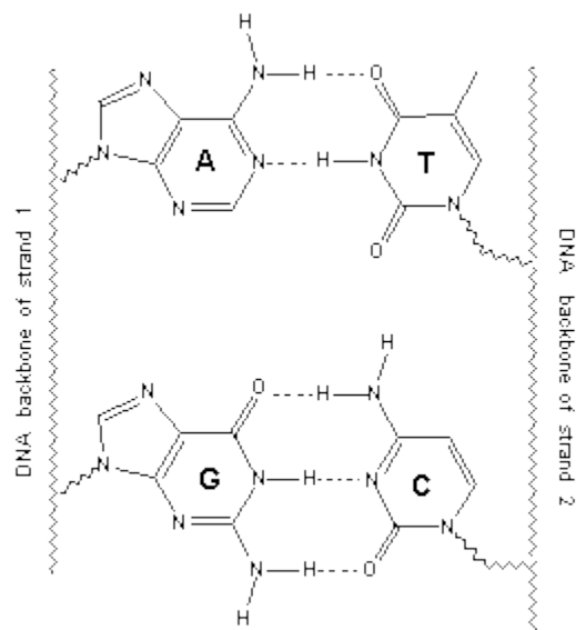
Figure 13.48: Base Pairs in DNA
