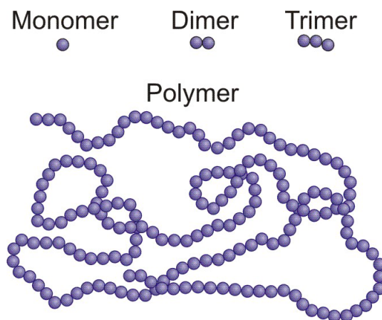
Figure 13.33: Several Mers
