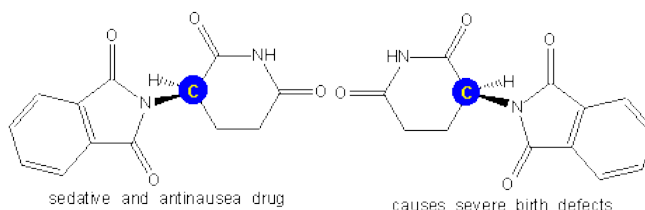
Figure 13.16: Thalidomide
