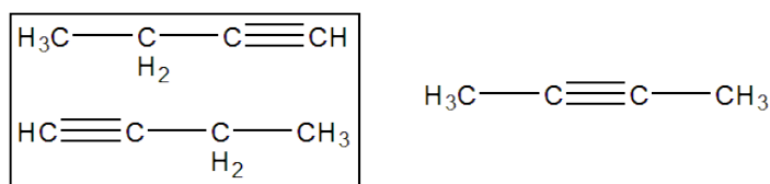
Figure 13.9: Isomers of Butyne
