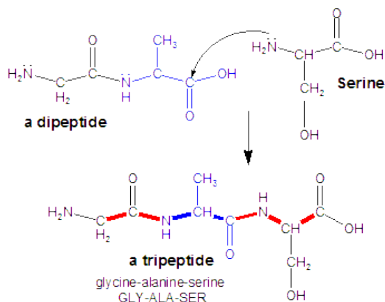
Figure 13.39b: Polypeptides: Tripeptide
