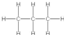
Figure 13.1b: Representations of Propane: Lewis Structure
