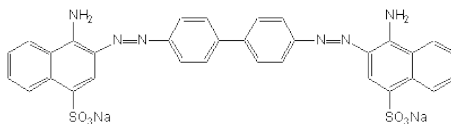
Figure 13.7b: Skeletal Structures of Two Polyenes: Congo Red
