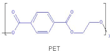
Figure 13.37c: Polyester Poly(ethylene terephthalate) or PET: Product
