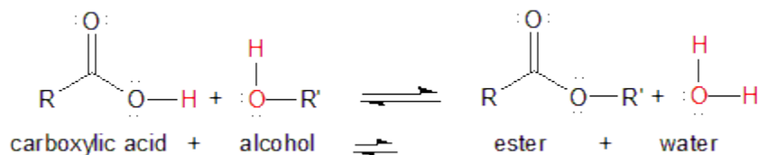
Figure 13.29: Esterification
