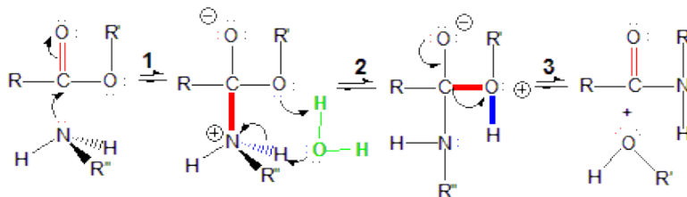
Figure 13.32: Amide Formation Mechanism
