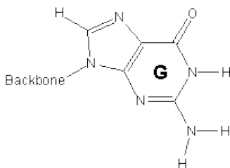
Figure 13.47: guanine (G)
