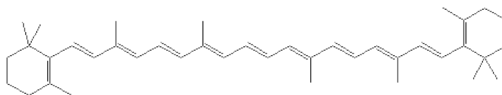
Figure 13.7a: Skeletal Structures of Two Polyenes: Beta Carotene
