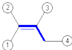
Figure 13.6: Possible Positions of the Fourth Carbon Atom in Butene
