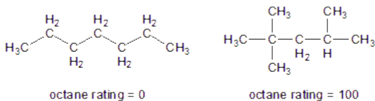
Figure 13.4: Reference Molecules Used to Determine Octane Ratings
