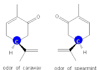
Figure 13.15: Carvone
