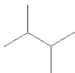
= 2,3-dimethylbutane
