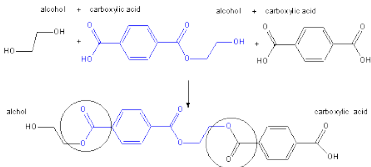
Figure 13.37b: Polyester Poly(ethylene terephthalate) or PET: Step 2
