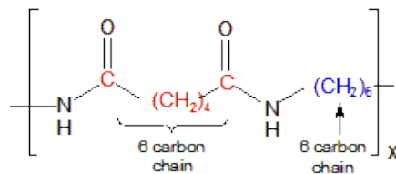
Figure 13.38b: Nylon 66
