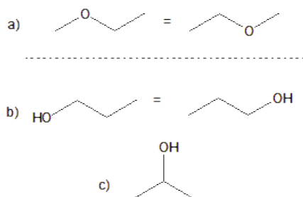
Figure 13.10: Isomers of C_3H_8O
