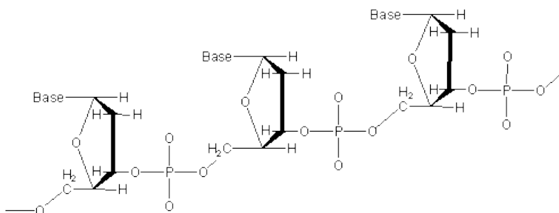
Figure 13.43: Three Residues of a DNA Molecule
