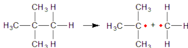
Figure 13.3: Free Radicals
