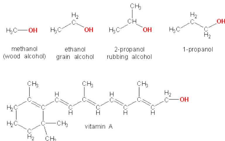
Figure 13.18: Some Common Alcohols
