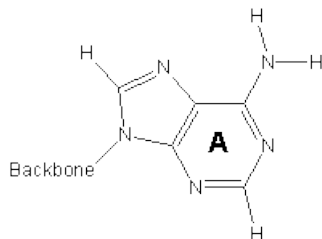
Figure 13.44: adenine (A)
