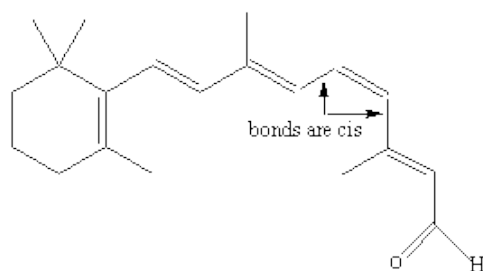
Figure 13.13a: Cis-Trans Isomerization in Retinal: Cis Isomer
