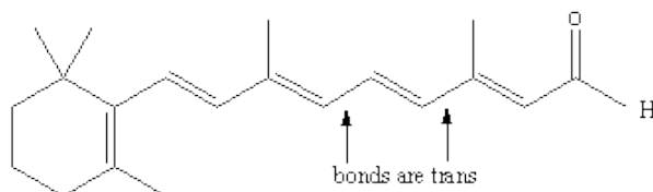
Figure 13.13b: Cis-Trans Isomerization in Retinal: Trans Isomer
