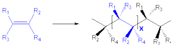
Figure 13.34: Alkene Polymerization
