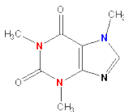
Figure 13.26: Caffeine
