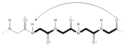
Figure 13.40: H-Bonds Responsible for the \alpha -helix Structure
