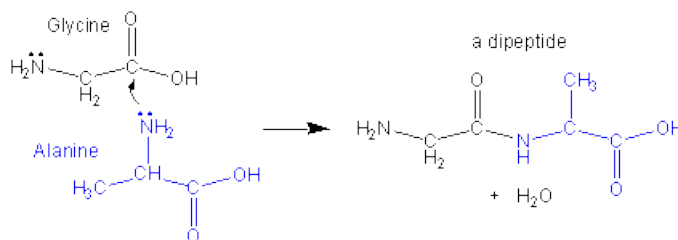
Figure 13.39a: Polypeptides: Dipeptide
