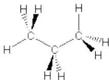
Figure 13.1a: Representations of Propane: Wedge-Dash
