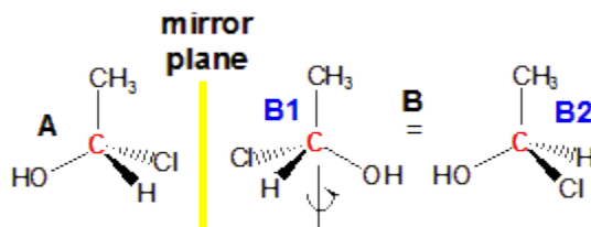
Figure 13.14: Enantiomers
