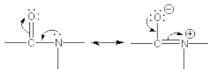
Figure 13.25: Amides
