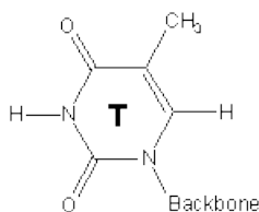
Figure 13.45: thymine (T)
