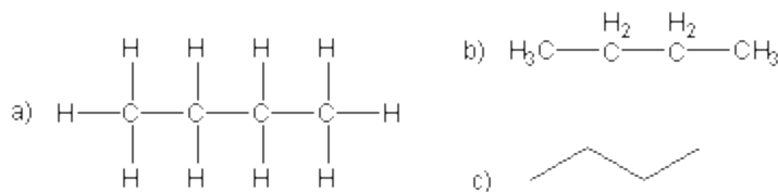
Figure 13.2a: Isomers of Butane: Straight Chain
