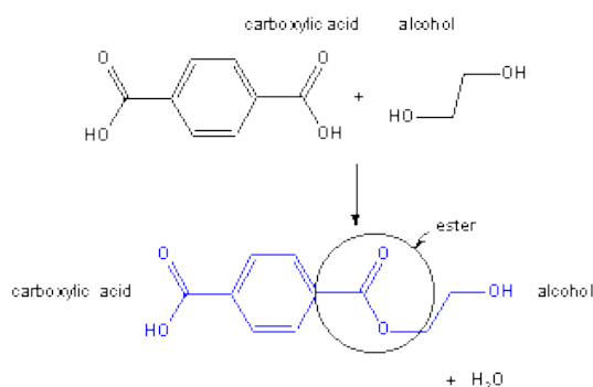
Figure 13.37a: Polyester Poly(ethylene terephthalate) or PET: Step 1
