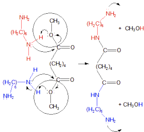
Figure 13.38a: Nylon
