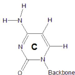
Figure 13.46: cytosine (C)
