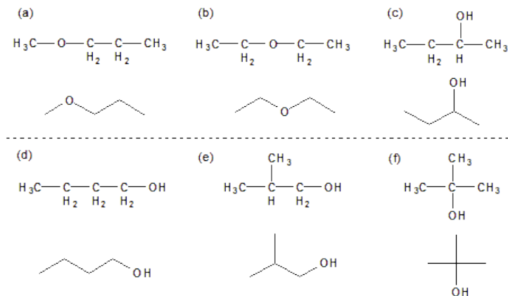
Figure 13.11: Isomers of C_4H_{10}O
