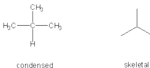
Figure 13.2b: Isomers of Butane: Branched Chain
